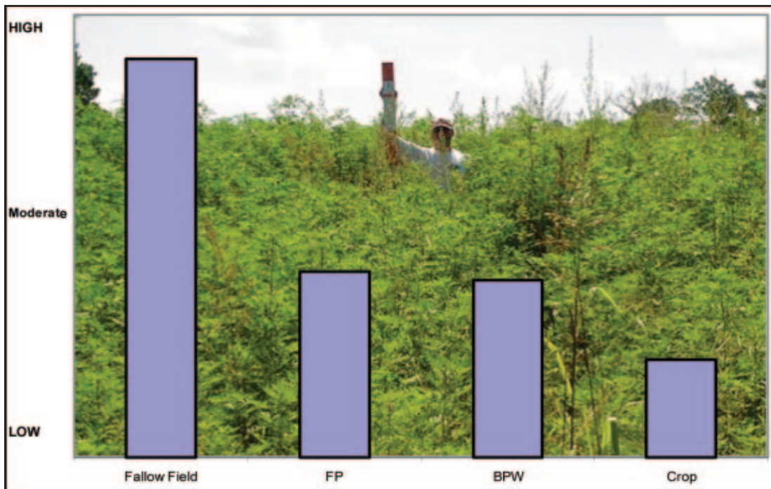
Figure 1: Insect populations rated on low to high scale for Fallow fields, Feed Patches, Burned Piney woods (bpw), and Crops. The background picture is a fallow fertilized ragweed field with an eight foot density board held by a 6'3" field technician.
